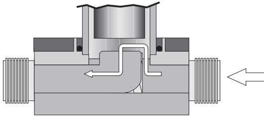
Fig. 2: Valve OPEN
