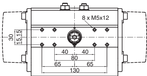
Detail X ADA/ASR 0020U-1750U
