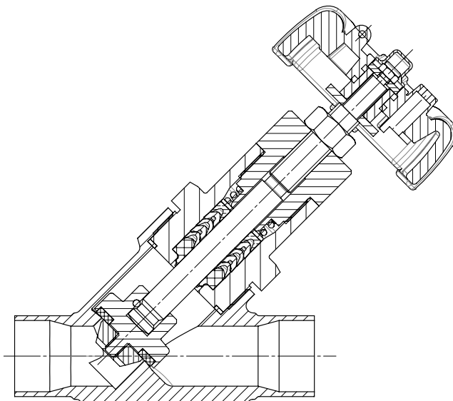
Sectional drawing
