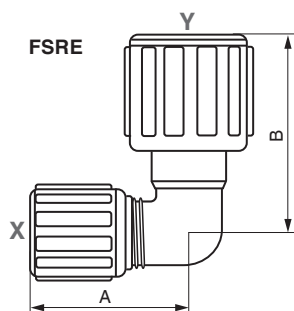
Reducer elbow, flare/space saver, PFA
