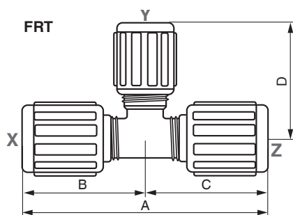
Union reducer tee, flare, PFA
