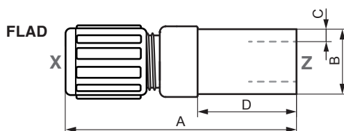
Straight adapter, flare/butt weld spigot, PVDF (max. 120 °C)
