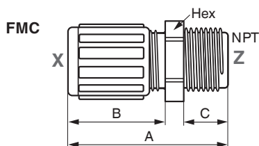
Straight adapter, flare/NPT male thread, PFA
