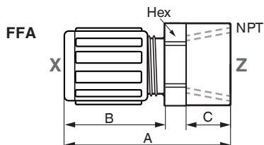
Straight adapter, flare/NPT female thread, PFA
