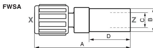
Straight adapter, space saver/butt weld spigot, PFA
