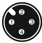
4-pin M12 built-in socket, A-coded
