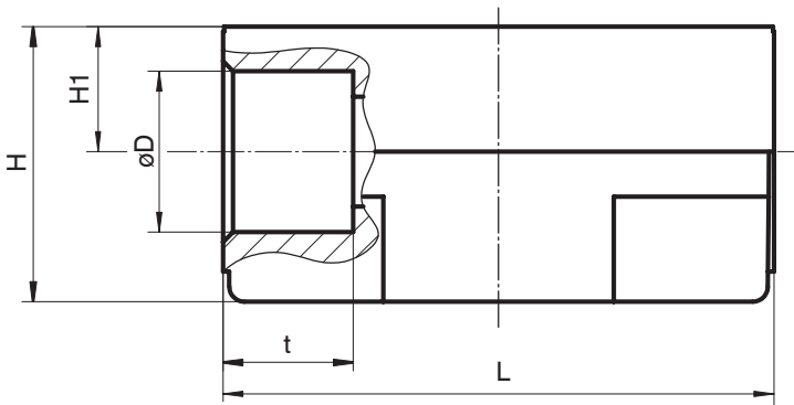
Connection type solvent cement socket (code 2) 1) , body material PVC-U (code 1) 2)
