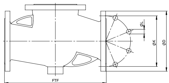
DN 50
