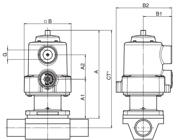
Control function 2 + 3 - Diaphragm size 10 Actuator size B/N
