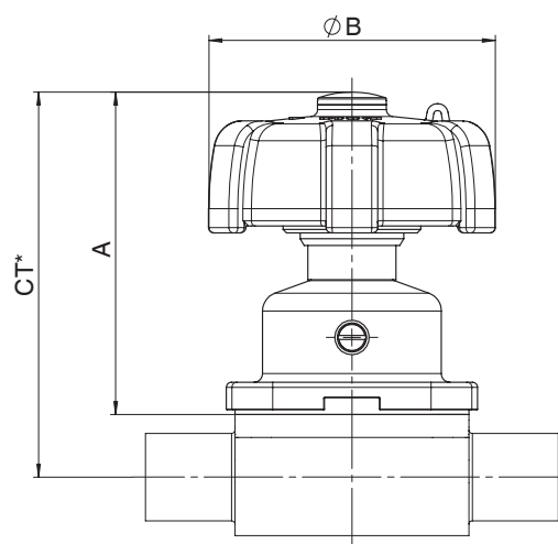
Diaphragm size 25 - 50
