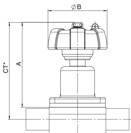
Diaphragm size 10
