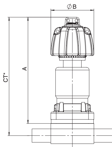
Diaphragm size 8
