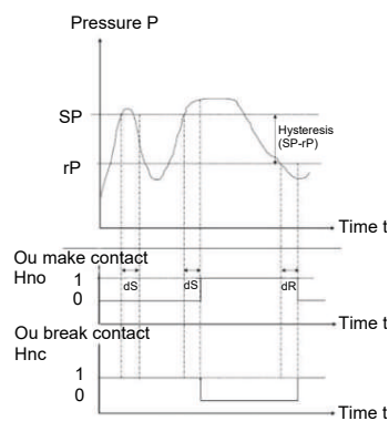
Fig. 3: Switching and switch-back delay for the hysteresis function in the pressure-time diagram
