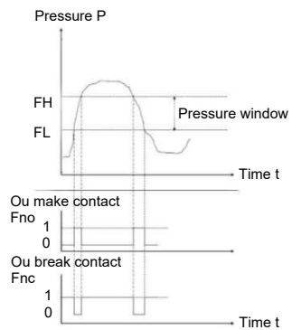
Fig. 4: Switching and switch-back characteristics for the window function in the pressure-time diagram
