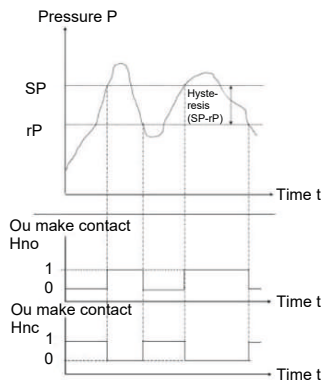
Fig. 2: Switching and switch-back characteristics for the hysteresis function in the pressure-time diagram
