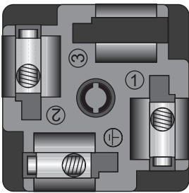
Fig. 4: Rear of terminal block
