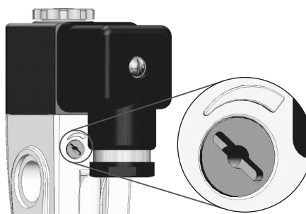
Fig. 5: Manual override
