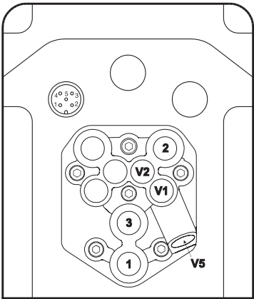
Pneumatic connections
