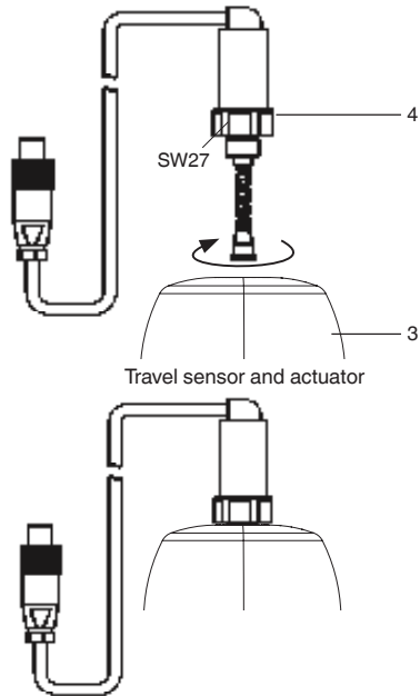
Travel sensor mounted to the actuator
