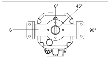
View X with mounting bracket and adapter
