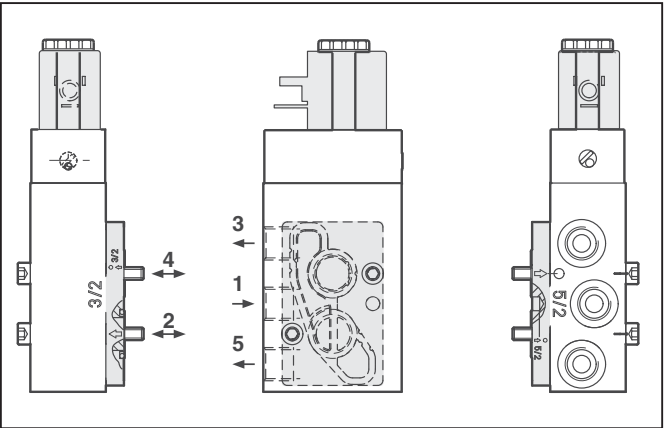
Raccords
