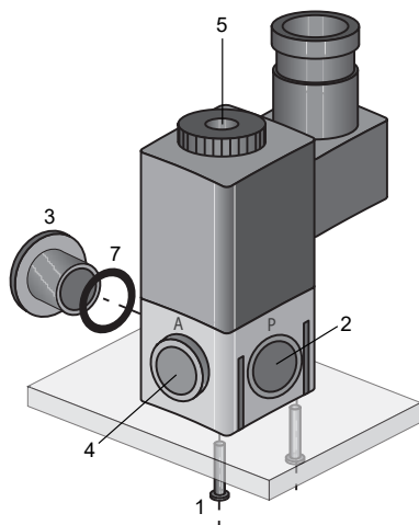
Fig. 1: Single mounting - GEMÜ 0322
