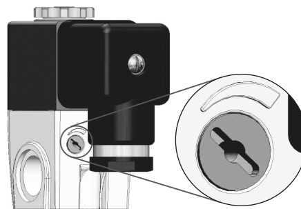
Fig. 5: Manual override
