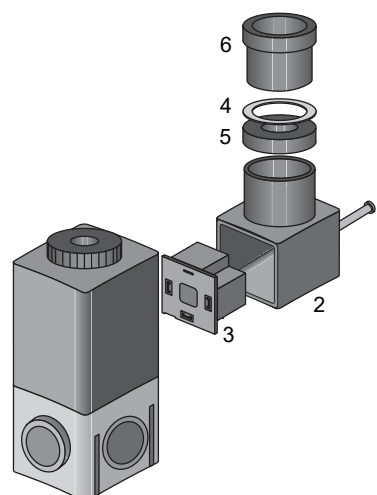
Fig. 3: Electrical connection of plug
