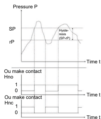
Fig. 2: Switching and switch-back characteristics for the hysteresis function in the pressure-time diagram
