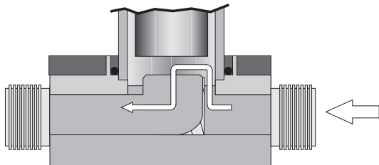
Fig. 2: Valve OPEN
