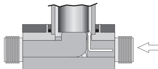
Fig. 1: Valve CLOSED
